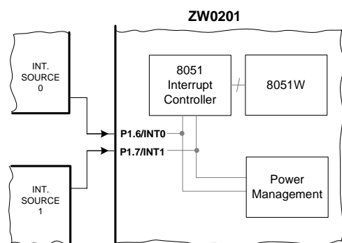
Figure 10: External interrupts
